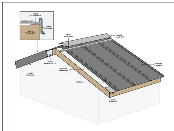
APEX ROOF
