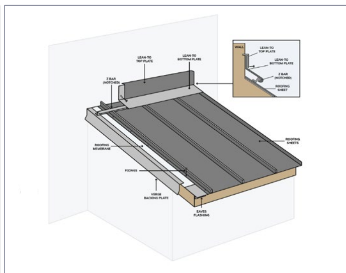
LEAN-TO ROOF
