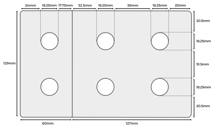
FLAT PROFILE
