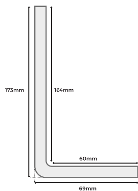
FORMED PROFILE
