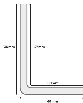
FORMED PROFILE
