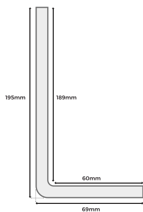
FORMED PROFILE
