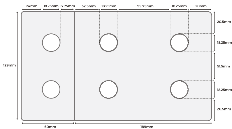
FLAT PROFILE
