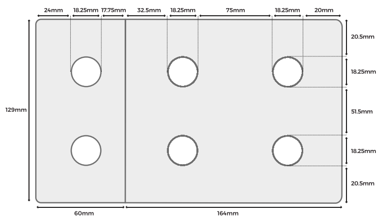
FLAT PROFILE
