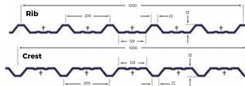
32/1000 Box Profile for roofing (0.7mm) or side cladding (0.5mm) (32mm height, 1000mm actual width coverage when lapped)
