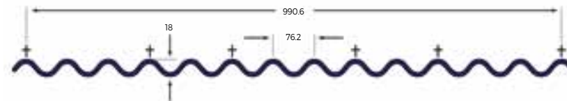
13/3 Corrugated Profile for roofing (0.7mm) or side cladding (0.5mm) (18mm profile height, 990mm actual width coverage when lapped)
