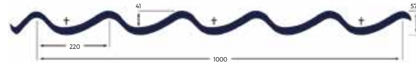
41/1000 Tile Form, pantile profile (41mm height, 1000mm actual width coverage when lapped)
